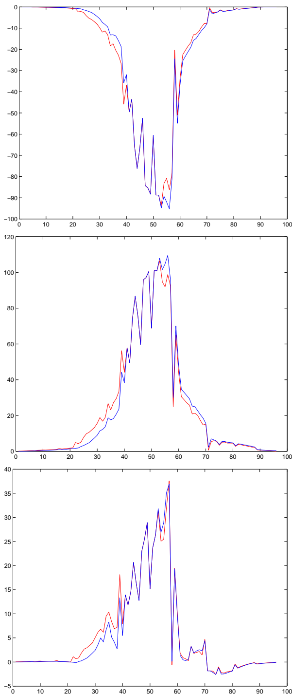
Figure 6. Haptic force along X, Y and Z (100 = 0.2N) calculated by the deformable loop (red) and by the latest haptic loop before the update (blue) during 100 steps of contact
