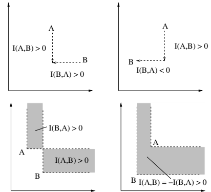
Fig. 5. Illustration of binary quality indicators for a two-objective minimization problem (top: I_{\epsilon+} -indicator, bottom: I_{HD} -indicator)
