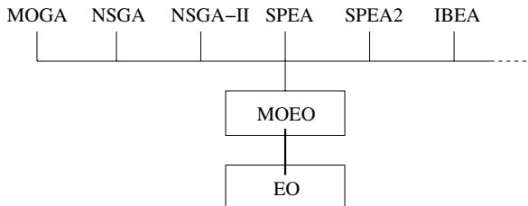
Fig. 1. Pareto-based multi-objective fitness assignment strategies proposed in EO and MOEO: MOGA, NSGA, NSGA-II, SPEA, SPEA2, IBEA, ...
