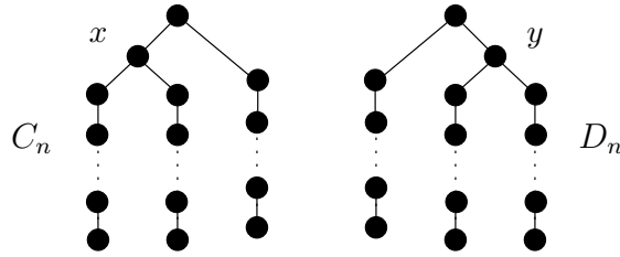
Fig. 2. Edit distance versus alignment 2. For each natural number n , define the trees C_n and D_n of height n + 1 and of size 3n + 2 as displayed above. This family of trees shows that the difference between the distance and the optimal alignment can be linear in the size of the trees. The value of the edit distance between C_n and D_n does not depend of n : the optimal mapping is composed of the deletion of x followed by the insertion of y . As for the optimal alignment, the cost is in O(n) , since it involves at least n - 1 deletions.
